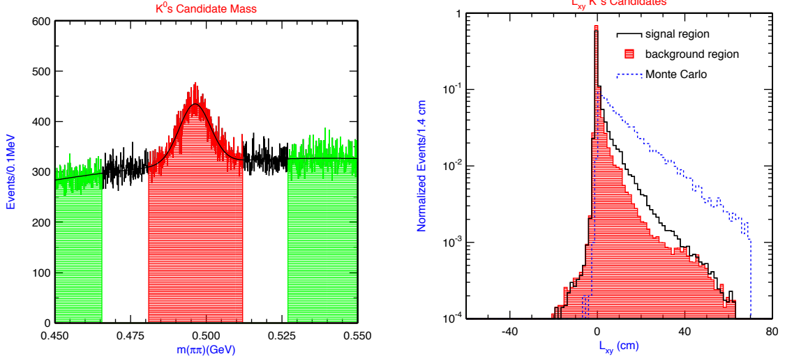
Figure 4.7: Left: K_s^0 mass distribution for K_s^0 candidates in the J/\psi sample: We require Prob(\chi^2) > 0.001 , p_T(\pi) > 400 MeV, and 5.1 < m_{\mu\mu\pi\pi} < 5.5 GeV. The shaded regions are the signal and background regions. Right: L_{xy}(K_s^0) for signal region, background region, and signal Monte Carlo. For the B^0 sample we require L_{xy} > 0.25 cm.
