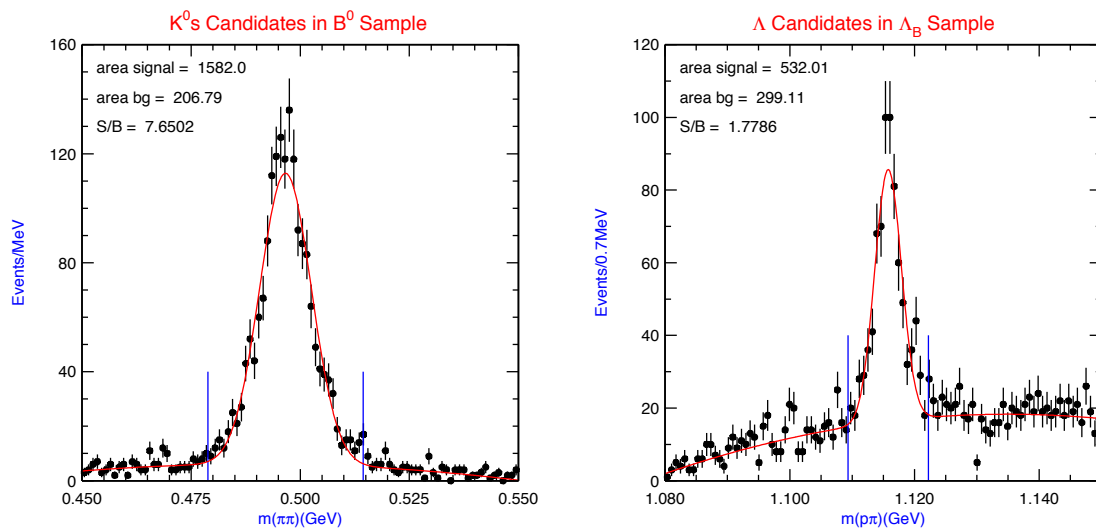
Figure 4.16: K_s^0 candidates in the B^0 sample (left) and \Lambda candidates in the \Lambda_B sample with all analysis requirements, excluding those on the K_s^0 and \Lambda invariant mass. All requirements are listed in Table 4.4. For the K_s^0 plot we require that the mass of the B^0 is between 5.1 and 5.5 GeV. For the \Lambda plot we require that the mass of the \Lambda_B is between 5.4 and 5.8 GeV.
