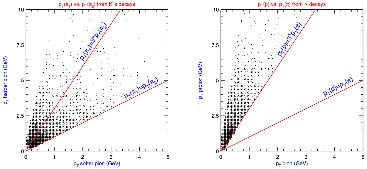
Figure 4.2: p_T of proton vs. p_T of pion in \Lambda decay and p_T of high momentum pion vs. p_T of low momentum pion in K_s^0 decay. The plot on the left shows p_T(\pi_1) vs. p_T(\pi_2) from K_s^0 decay. \pi_1 is the pion with larger p_T . The plot on the right shows p_T(p) vs. p_T(\pi) from \Lambda decay. Plots are from B^0 \rightarrow J/\psi K_s^0 and \Lambda_b \rightarrow J/\psi\Lambda Monte Carlo generated without simulation. Lines drawn on the plots represent y = x and y = 3x .
