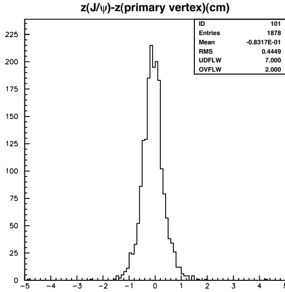
Figure 5.1: Distribution of z_{J/\psi} - z(\text{primary vertex}) for B^0 candidate events. We use the primary vertex which is closest in z to the J/\psi vertex.
