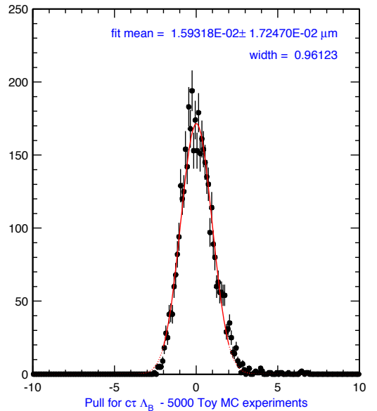
Figure 5.9: Results for lifetime fits to 5000 toy Monte Carlo experiments. The top two plots show the distributions of fitted lifetime for B^0 and \Lambda_B . The bottom two plots show the pull on the lifetime.
