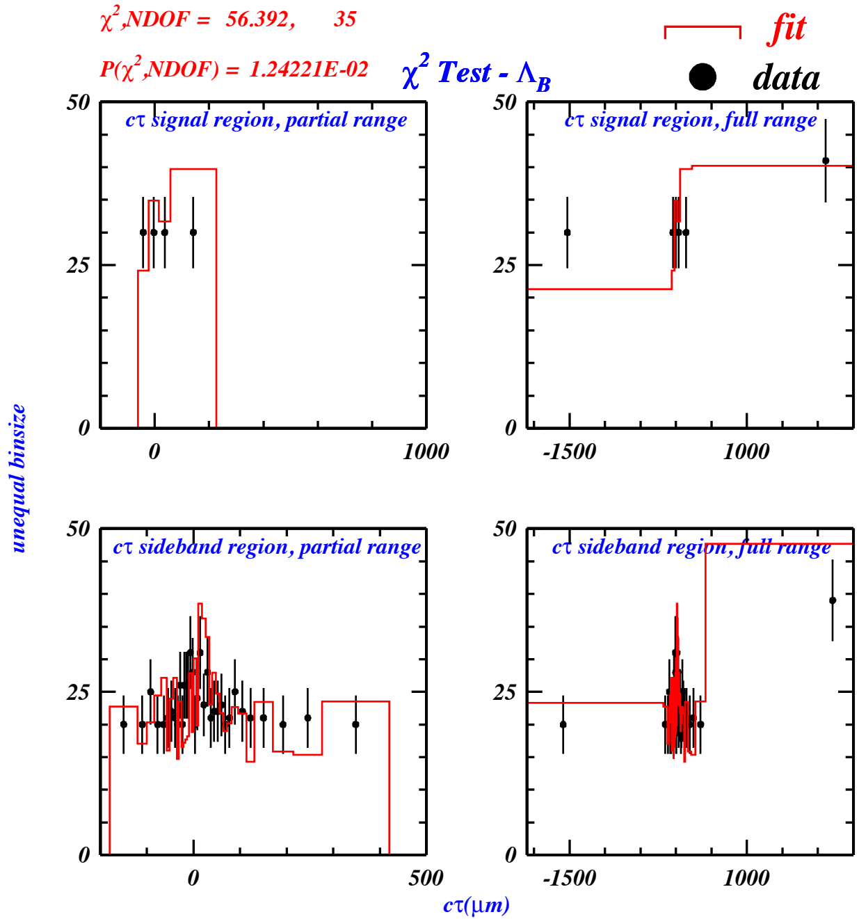
Figure 5.13: \chi^2 test for Goodness of Fit, for the \Lambda_B lifetime. The data are the points with error bars, and the fit is shown in the overlaid histogram. We have varied the binsize so that each bin contains at least 20 events. The top plots show the signal region, and the bottom show the sideband region. Plots on the left show a subset of the entire range, and plots on the right show the entire range.
