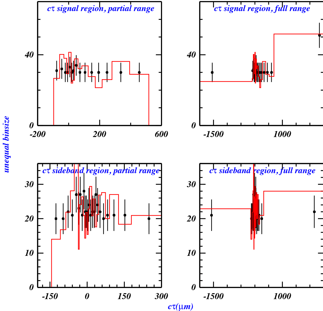
Figure 5.12: \chi^2 test for Goodness of Fit, for the B^0 lifetime. The data shown here are from the final sample. The data are the points with error bars, and the fit is shown in the overlaid histogram. We have varied the binsize so that each bin contains at least 20 events. The top plots show the signal region, and the bottom show the sideband region. Plots on the left show a subset of the entire range, and plots on the right show the entire range.
