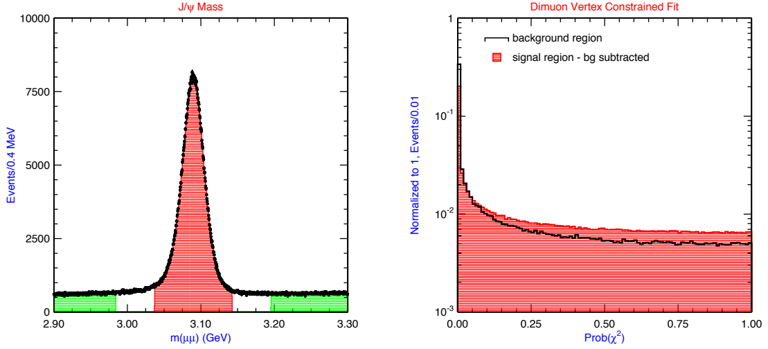
Figure 4.3: J/\psi mass distribution, from the J/\psi sample (left), showing signal region and sideband (background) region in the shaded areas. Distribution of Prob(\chi^2) (right) for vertex constrained dimuon fit, for signal and background. The histograms at the right are normalized to unit area.
