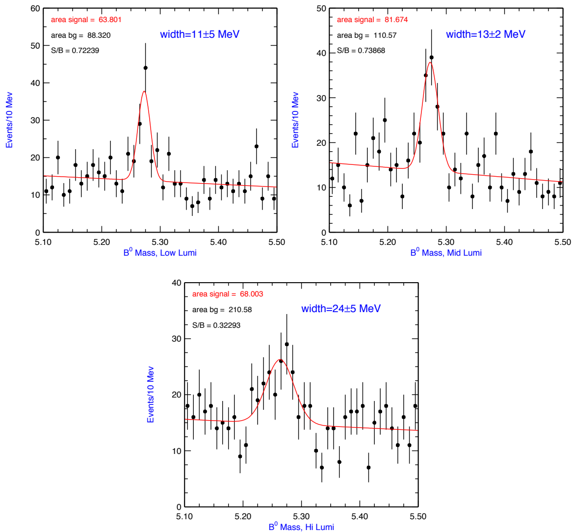
Figure 6.5: Width of the B^0 mass peak in 3 regions of instantaneous luminosity. We divide the data at 1.170 \times 10^{31} and 1.7 \times 10^{31} \text{ cm}^{-2} \text{ s}^{-1}
