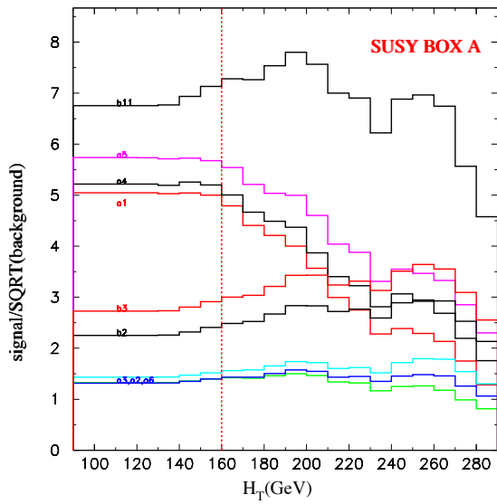
Figure H.19: H_T Optimization Box A.
