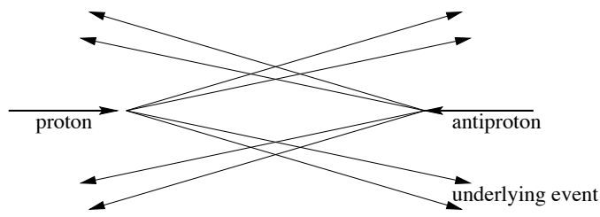
Figure 6.3: Schematic of Hard (a), Multiple (b), and Soft (c) interactions in proton antiproton collisions.
