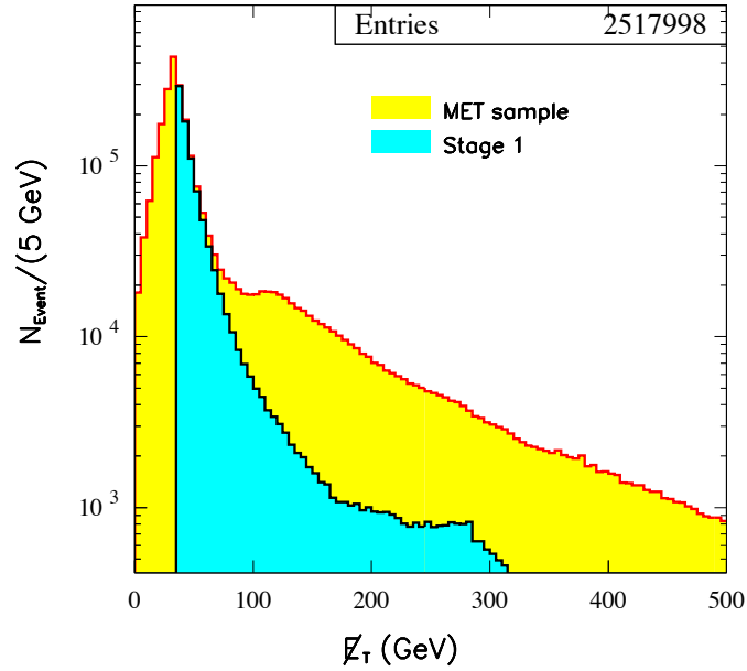
Figure 4.5: \cancel{E}_T spectrum before and after Stage 1 of the Pre-Selection.
