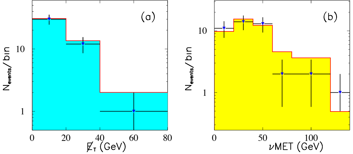
Figure 5.6: Comparison between data and normalized Z(\rightarrow e^+e^-)+\geq 3 ELO Monte Carlo of the (a) \cancel{E}_T and (b) \nu\cancel{E}_T in the inclusive 3 jet bin.
