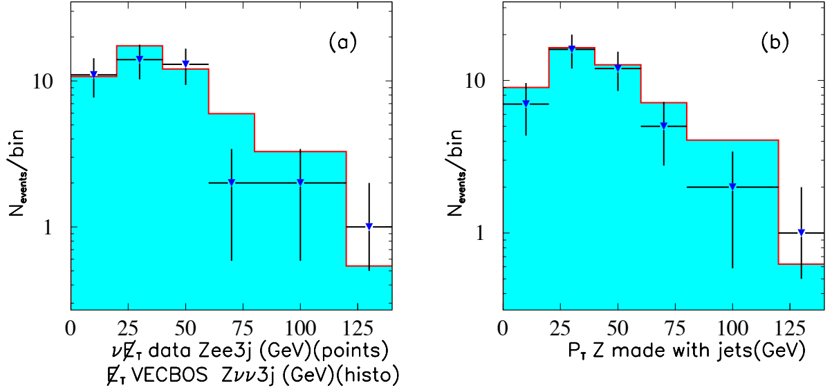
Figure 5.4: (a) \nu \cancel{E}_T in the Z(\rightarrow e^+e^-) + 3 jet data sample compared with the \cancel{E}_T in the ELO Z(\rightarrow \nu\bar{\nu}) + \geq 3 jets Monte Carlo. (b) Z P_T comparison of the same samples. The boson P_T is the jet \sum \vec{E}_T .
