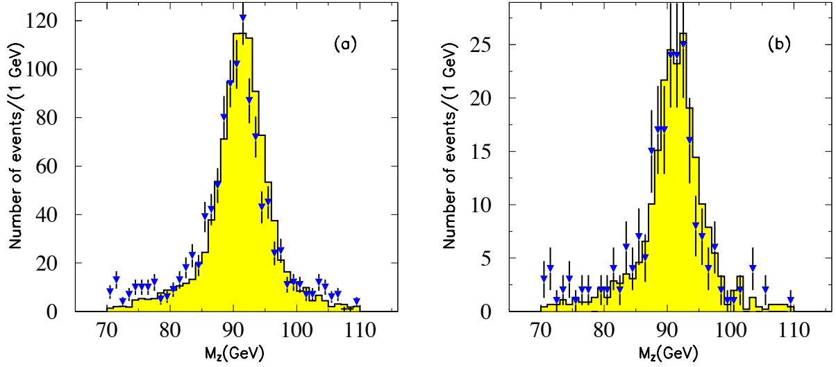
Figure E.1: Z mass in inclusive jet multiplicity bins 1 and 2 as predicted in Z \rightarrow ee + \geq 1 jet Enhanced LO Monte Carlo (histogram) compared with data (points).
