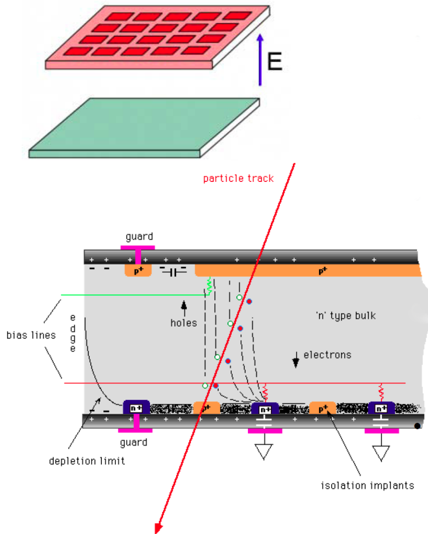
Figure 3.8: Silicon detector operating principles [5].
