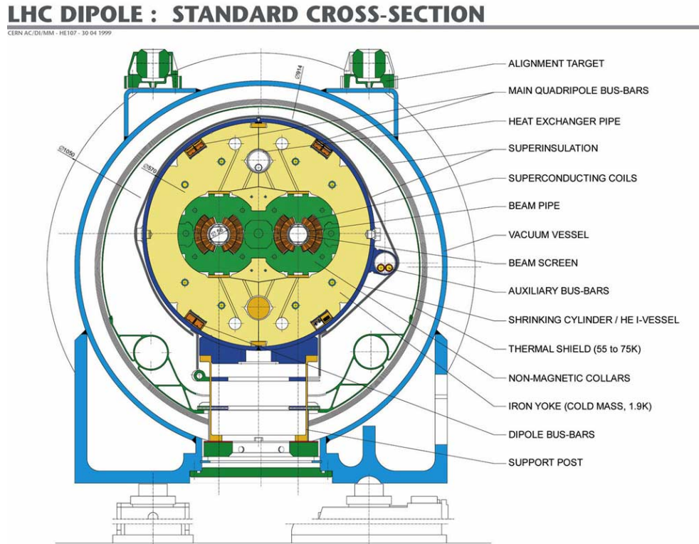
Figure 3.2: Cross section of a LHC dipole magnet [3].
