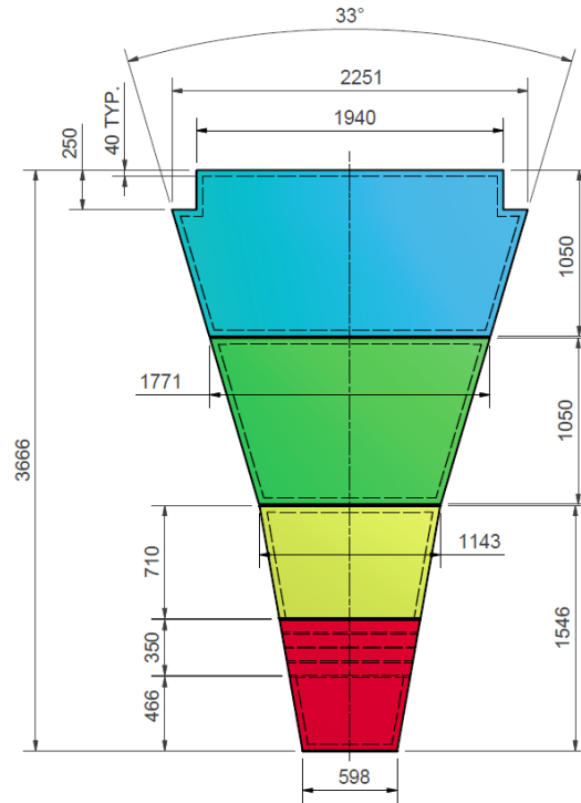
Figure 4.7: A single sector of the 2012 NSW where a sector is defined as 1/16 of the NSW on either side A or C comprised of sTGC and MM wedges [52].
