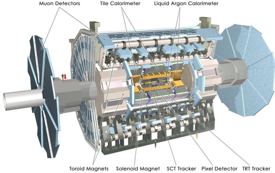
Figure 3.4: Cross sectional view of the ATLAS detector [22].
